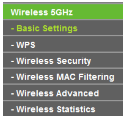
Figure 4-29 Wireless menu
