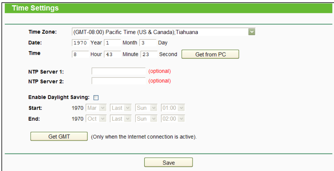
Figure 4-109 Time settings
